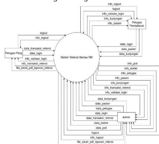
Gambar 4. Context Diagram/Diagram Level 0
