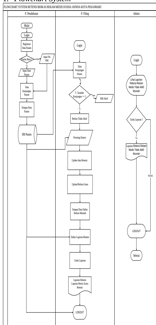
Gambar 3. Flowchart System
