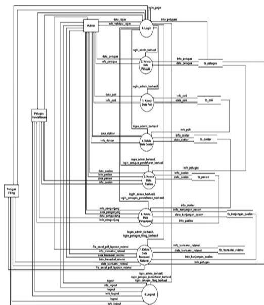
Gambar 5. Data Flow Diagram (DFD)
